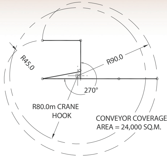
PLAN OF CONVEYOR COVERAGE
